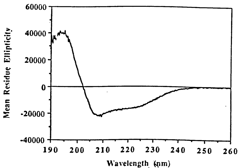
FIG. 4. Far ultraviolet CD spectra of a 6:1 SDS-insulin complex in neat 1-octanol. The pathlength was 1mm. The insulin concentration was 61 \mu\text{g}/\text{ml} for the sample at 5° C.
